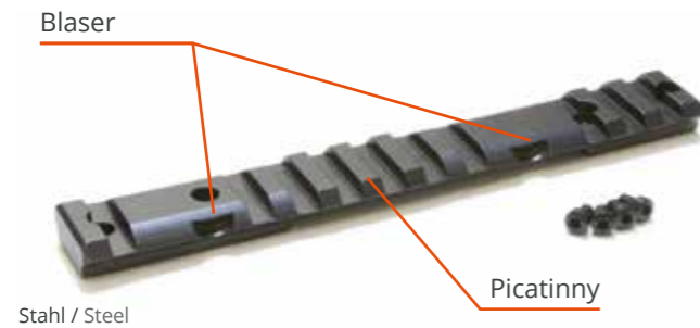
Stahl / Steel
